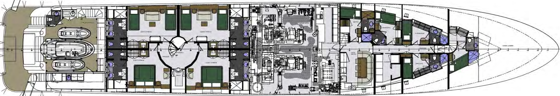
PROPOSED LOWER DECK
