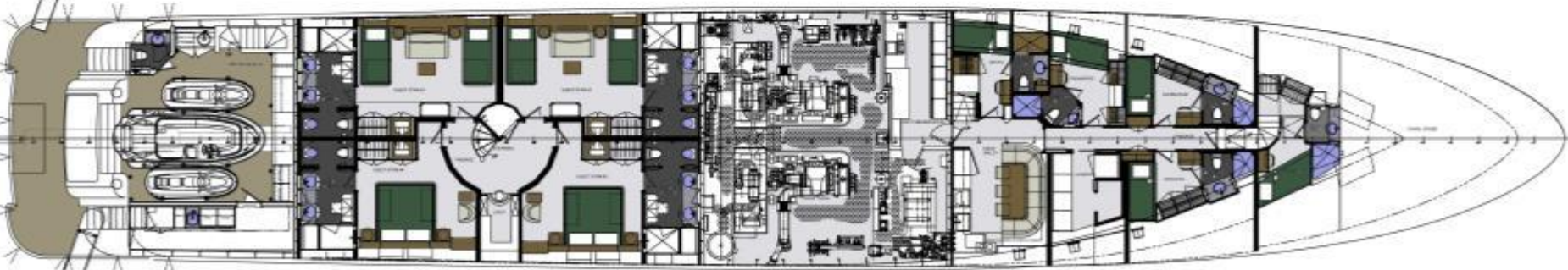
PROPOSED LOWER DECK SCALE: 3/16"=1'-0"
