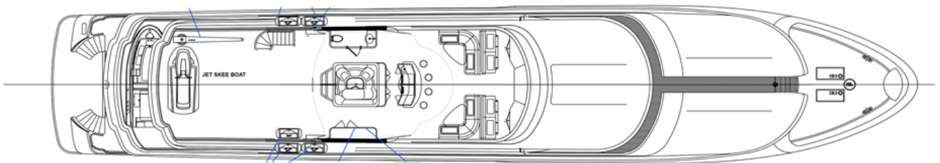
FLYBRIDGE PLAN "F"
