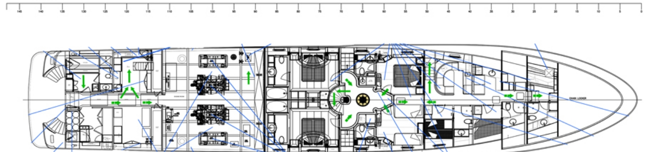
LOWER DECK PLAN "L"
