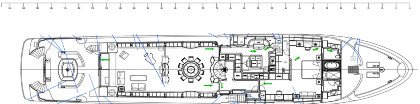
MAIN DECK PLAN "M"
