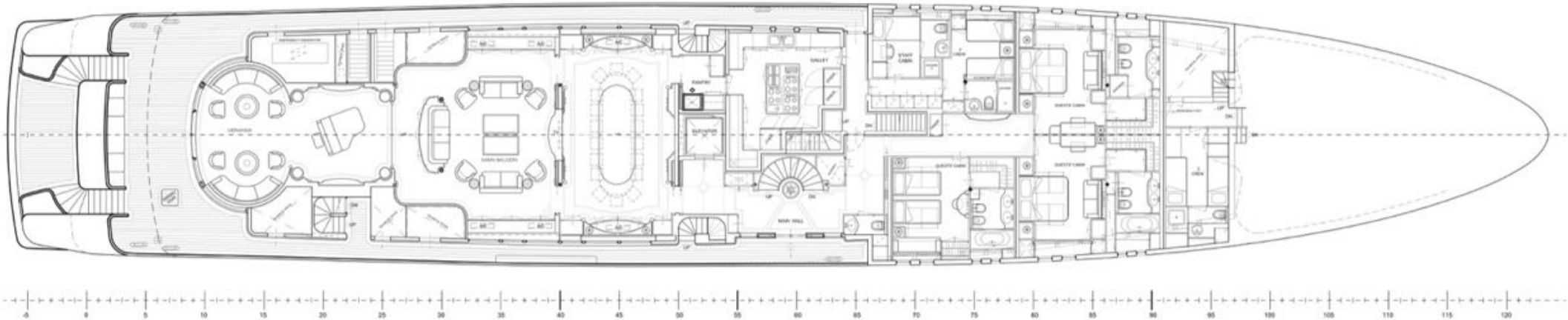
MAIN DECK
