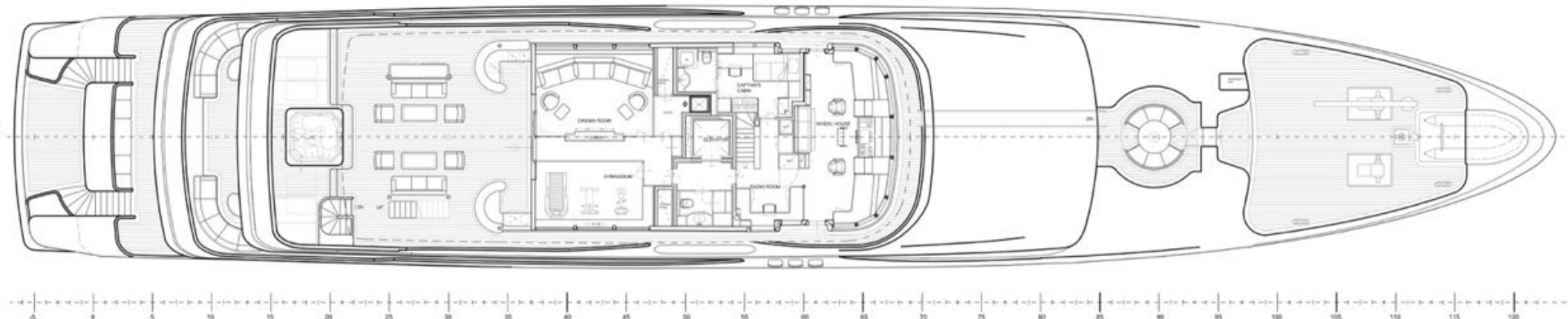
BRIDGE DECK
