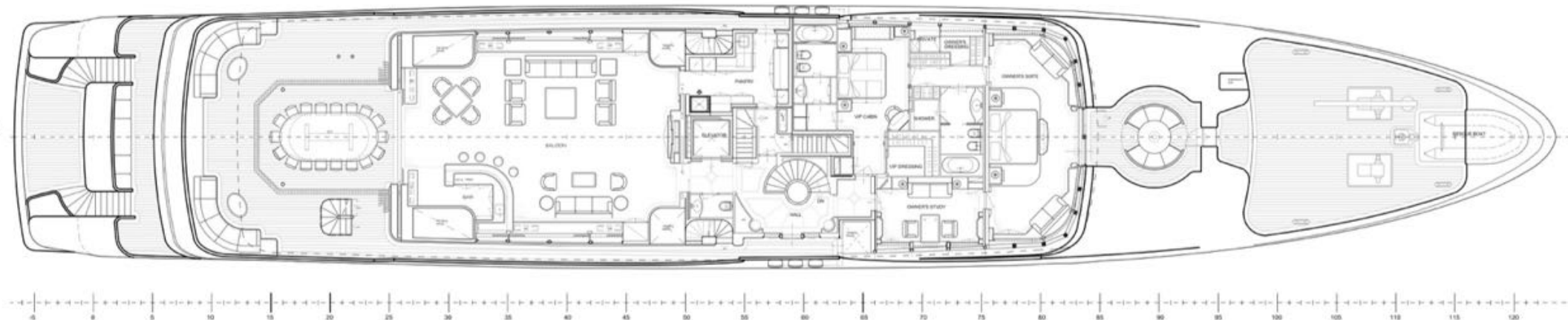
UPPER DECK
