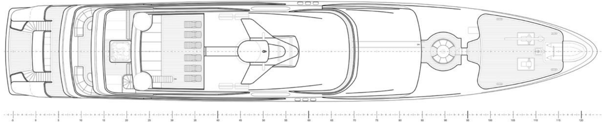
SUN DECK
